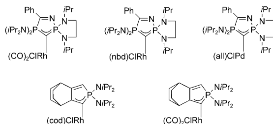
Scheme 53. Complexes synthesized from free CCDP 4 and CVP 2 . all = allyl.
