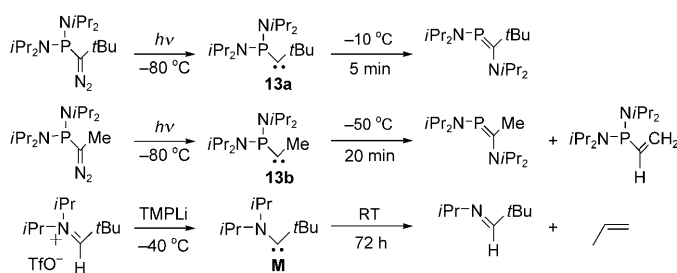
Scheme 14. Evolution of persistent (alkyl)(phosphino)- and (alkyl)-(amino)carbenes in solution.
