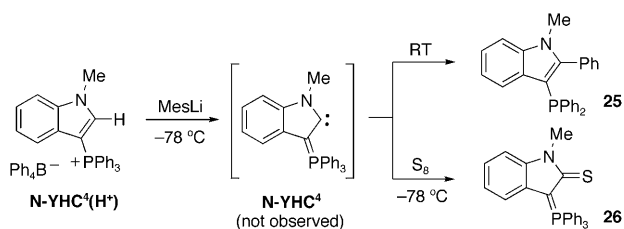
Scheme 31. Generation, rearrangement, and trapping of N-YHC 4 .
