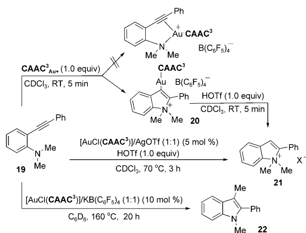
Scheme 26. Isolation of gold(I)–( \eta^1 -alkene) complex 20 , as well as examples of catalytic hydroammonium and methylamination reactions to give 21 and 22 , respectively.
