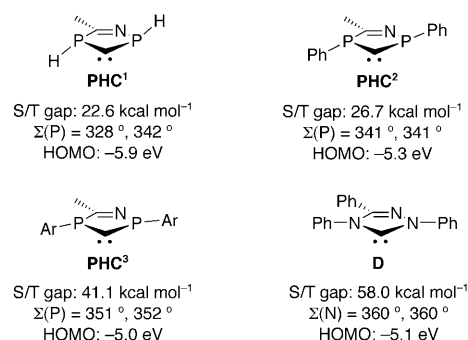
Scheme 4. Computational data for PHC 1-3 and triazolin-5-ylidene D . S = singlet, T = triplet.
