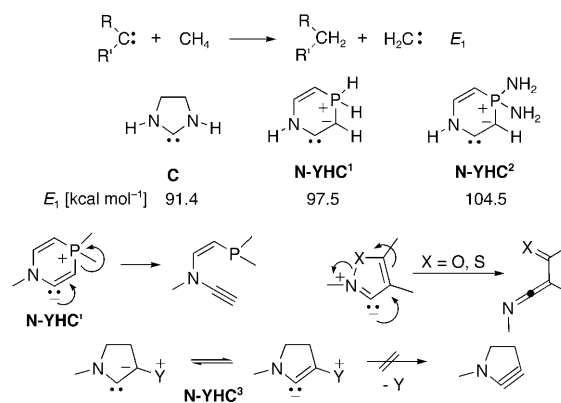
Scheme 30. The E_1 value correlates with the nucleophilicity of the carbenes. The cationic part of the ylide has to be exocyclic to prevent ring-opening processes, as observed for other cyclic carbenes.
