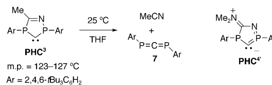
Scheme 8. Decomposition of \text{PHC}^3 in solution, and resonance form \text{PHC}^4 .
