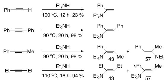
Scheme 22. Hydroamination of alkynes with diethylamine by using 5 mol% CAAC 3 Au+ .
