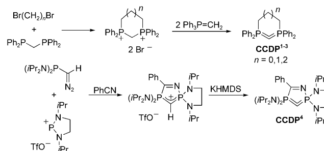
Scheme 49. Syntheses of cyclic carbodiphosphoranes CCDP 1-4 .
