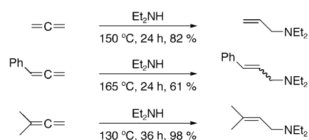
Scheme 23. Hydroamination of allenes with diethylamine by using 5 mol% CAAC 3 Au+ .
