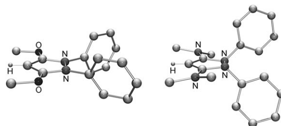
Figure 11. Molecular structures of CBA 3 (H + ) (left; the Dipp groups on the oxygen atoms have been removed for clarity), and CBA 4 (H + ) (right) in the solid state.
