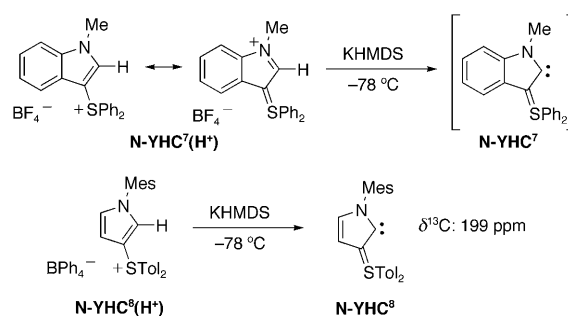
Scheme 34. Preparation of the transient N-YHC 7 and persistent N-YHC 8 , showing the importance of the ring skeleton.
