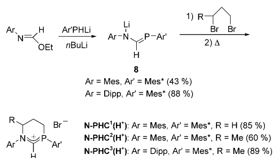
Scheme 11. Synthesis of phosphoramidates 8 and N-PHC 1-3 (H + ) . Mes = 2,4,6-Me 3 C 6 H 2 , Mes* = 2,4,6- t Bu 3 C 6 H 2
