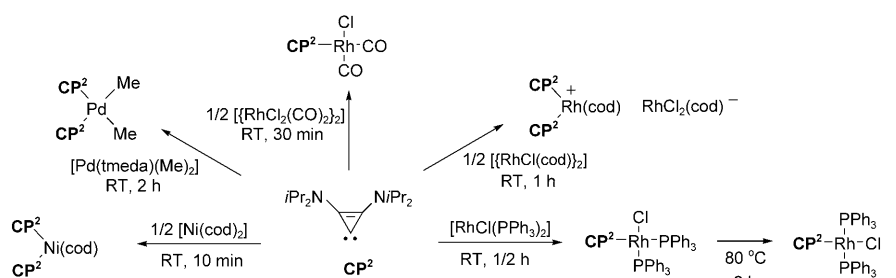
Scheme 41. Complexes prepared from free \text{CP}^2 . tmeda = N,N,N',N' -tetramethylethylenediamine.
