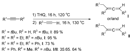
Scheme 24. One-pot synthesis of allenes from two alkynes and a sacrificial amine by using 5 mol % CAAC 3 Au+ . THQ = 1,2,3,4-tetrahydroisoquinoline.
