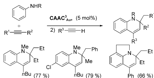
Scheme 25. Tandem hydroamination-hydroarylation reaction, promoted by CAAC 3 Au+ .
