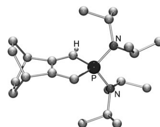
Figure 13. Molecular structure of CVP 2 in the solid state.
