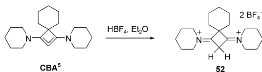
Scheme 48. Double protonation of CBA 5 .
