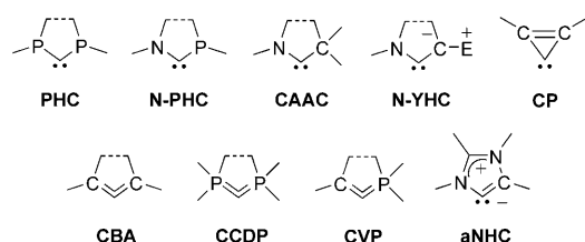
Scheme 3. Cyclic carbenes and related species discussed in this Review.
