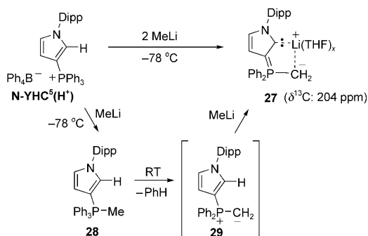
Scheme 32. Deprotonation of N-YHC 5 (H + ) affords stable lithium adduct 27 , which has an N-YHC as part of a bidentate ligand.
