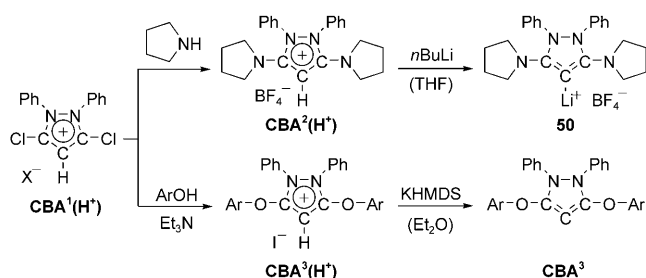
Scheme 46. Synthesis of CBA 2 -lithium adduct 50 , and stable free cyclic bent-allene CBA 3 . Ar = 2,6-Me 2 C 6 H 3 .
