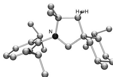
Figure 3. Solid-state structure of enantiomerically pure CAAC 2 .
