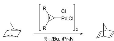
Scheme 42. Isomerization of quadricyclane to norbornadiene promoted by [\text{PdCl}_2(\text{CP})]_2 dimers.
