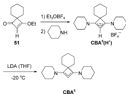
Scheme 47. Synthesis of CBA 5 (H + ) and persistent cyclic allene CBA 5 .
