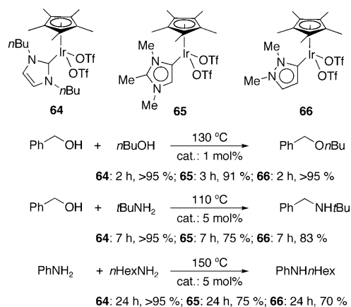
Scheme 62. Comparison of iridium complexes bearing NHC ( 64 ), aNHC ( 65 ), and pyrazol-3-ylidene ( 66 ) ligands for alkylation reactions.
