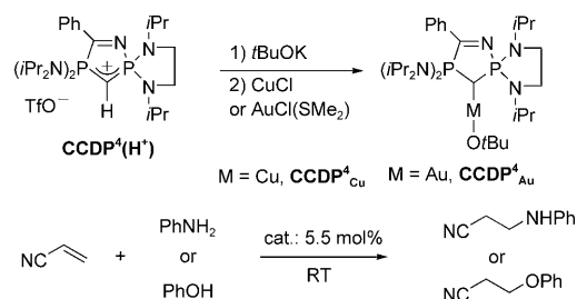
Scheme 54. First catalytic applications of complexes bearing a CCDP as a ligand.
