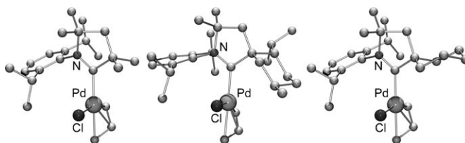
Figure 7. Solid-state structures of palladium complexes showing the different steric environments provided by small CAAC 1 (left), bulky rigid CAAC 2 (middle), and flexible CAAC 3 (right).
