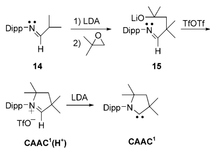
Scheme 15. First synthetic route for the preparation of the small CAAC 1 .
