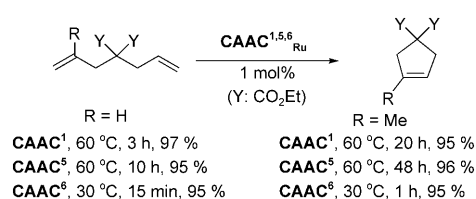
Scheme 28. Application of CAAC 1,5,6 Ru in ring-closing metathesis reactions.
