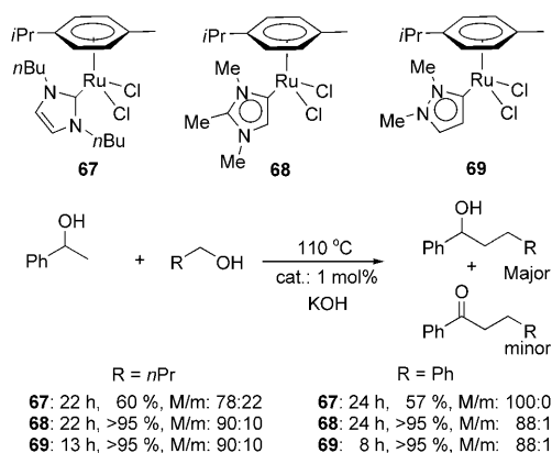
Scheme 63. Comparative activity of ruthenium complexes bearing NHC ( 67 ), aNHC ( 68 ), and pyrazol-3-ylidene ( 69 ) ligands for the \beta -alkylation of secondary alcohols with primary alcohols. M = major product, m = minor product.
