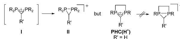
Scheme 5. Spontaneous ring closure of phosphorus analogues of amidinium salts, which can be prevented by the ring structure of PHC(H + )s.
