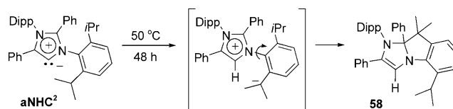
Scheme 59. Rearrangement of aNHC 2 upon heating in solution.
