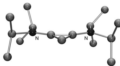
Figure 9. Solid-state structure of CP 2 .
