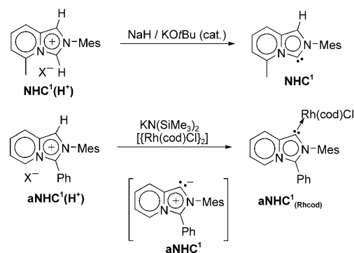
Scheme 57. Synthesis of NHC 1 , and evidence for the transient formation of aNHC 1 through the formation of aNHC 1 (Rhcod) . [163c]
