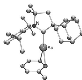
Figure 6. X-ray crystal structure of [\text{Au}(\text{CAAC}^3)(\eta^2\text{-toluene})]\text{B}(\text{C}_6\text{F}_5)_4 ( CAAC 3 Au+ ).
