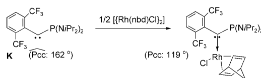
Scheme 2. Contraction of the carbene bond angle of K upon complexation. nbd = norbornadiene.
