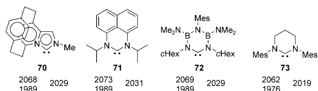
Scheme 65. Members of the NHC family reaching the donor strength of CBAs and N-YHCs.
