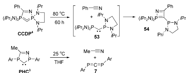
Scheme 50. Rearrangement of CCDP 4 ; analogy with PHC 3 .
