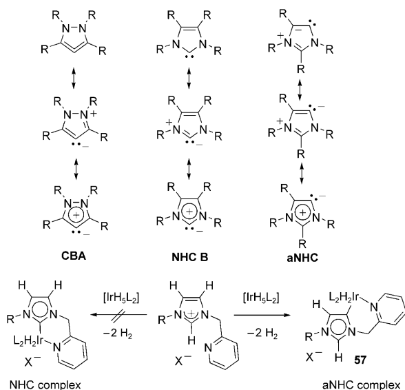
Scheme 56. Different resonance forms of CBA (derived from pyrazolium salts), NHC B , and aNHC . Synthesis of the abnormal NHC complex 57 .
