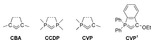
Scheme 51. Cyclic vinylidenephosphoranes (CVPs), which are hybrid compounds between CBAs and CCDPs; CVP 1 , the only derivative reported [210] before 2008.
