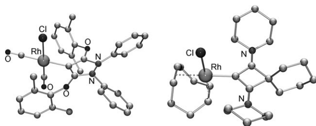
Figure 14. X-ray crystal structures of [\text{RhCl}(\text{CO})_2(\text{CBA}^3)] and [\text{RhCl}(\text{cod})(\text{CBA}^5)] .
