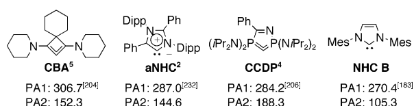
Scheme 66. Calculated first and second proton affinity [ \text{kcal mol}^{-1} ].
