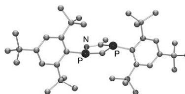
Figure 1. Solid-state structure of \text{PHC}^3 showing the very weak pyramidalization of the phosphorus centers.
