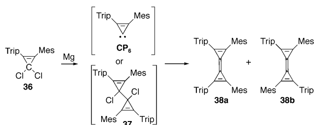
Scheme 40. Preparation of triafulvalenes 38 , and the possible reaction intermediates. Trip = 2,4,6- i -Pr 3 C 6 H 2 .
