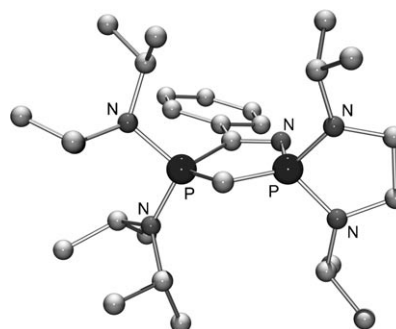
Figure 12. Solid-state structure of CCDP 4 .
