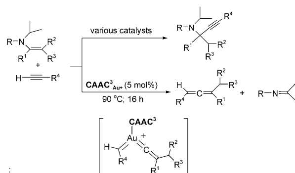
Scheme 20. Metal-catalyzed coupling of enamines and terminal alkynes.
