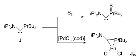
Scheme 10. Acyclic (amino)(phosphino)carbenes such as J feature an active lone pair of electrons on the P center. cod = 1,5-cyclooctadiene.
