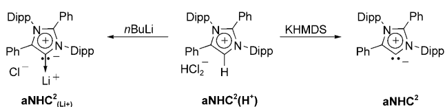
Scheme 58. Synthesis of free aNHC 2 and of its lithium adduct aNHC 2 (Li + ) .
