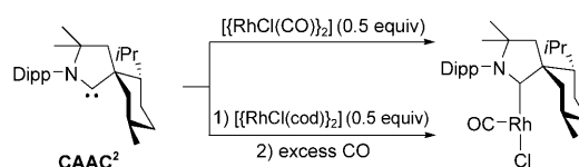
Scheme 19. Synthesis of 14-electron [RhCl(CO)( CAAC 2 )].
