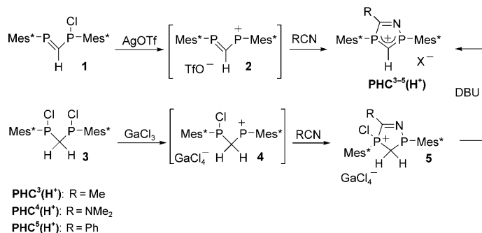
Scheme 6. Synthetic routes to \text{PHC}^{3-5}(\text{H}^+) . \text{Mes}^* = 2,4,6\text{-}t\text{Bu}_3\text{C}_6\text{H}_2 , \text{Tf} = trifluoromethanesulfonyl, \text{DBU} = 1,8\text{-diazabicyclo}[5.4.0]\text{undec-7-ene} .
