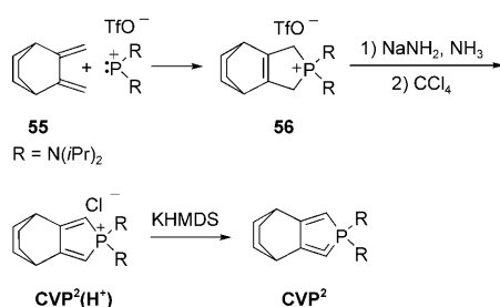
Scheme 52. Synthesis of CVP 2 .
