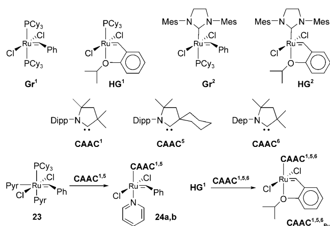
Scheme 27. Classical ruthenium olefin metathesis catalysts Gr 1,2 and HG 1,2 . CAAC 1,5,6 were used for preparing 24a,b , and CAAC 1,5,6 Ru.
