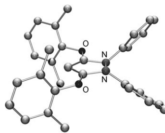
Figure 10. Molecular structure of CBA 3 in the solid state.
