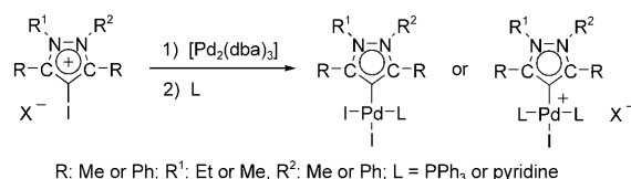
Scheme 55. Synthesis of complexes used for Suzuki–Miyaura coupling reactions. dba = trans,trans -dibenzylideneacetone.
