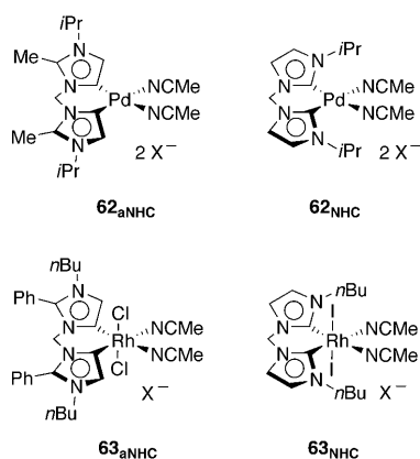
Scheme 61. aNHC complexes 62 aNHC and 63 aNHC are active in hydrogenation and hydrogen-transfer catalysis, respectively, while NHC complexes 62 NHC and 63 NHC are not.
