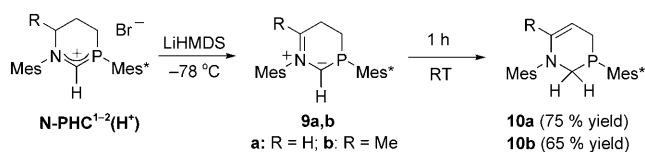
Scheme 12. Deprotonation of N-PHC 1,2 (H + ) .
