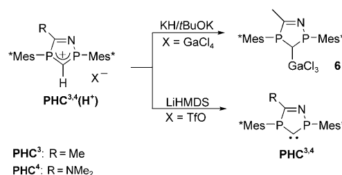
Scheme 7. Influence of the counteranion/base combination on the deprotonation of \text{PHCs} ; preparation of \text{PHC}^3 and \text{PHC}^4 . \text{Ar} = 2,4,6\text{-}t\text{Bu}_3\text{C}_6\text{H}_2 , \text{HMDS} = 1,1,1,3,3,3\text{-hexamethyldisilazane} .
